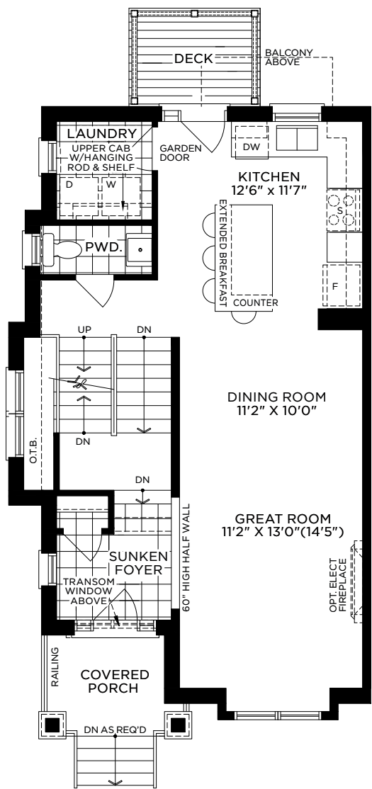
Corner Mod 2 Elev A Main Floor
