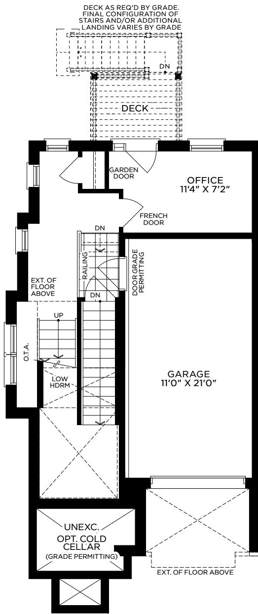
Corner Mod 2 Elev A, B Lower Floor
