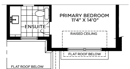
Mod 3 Elev B Upper Floor
