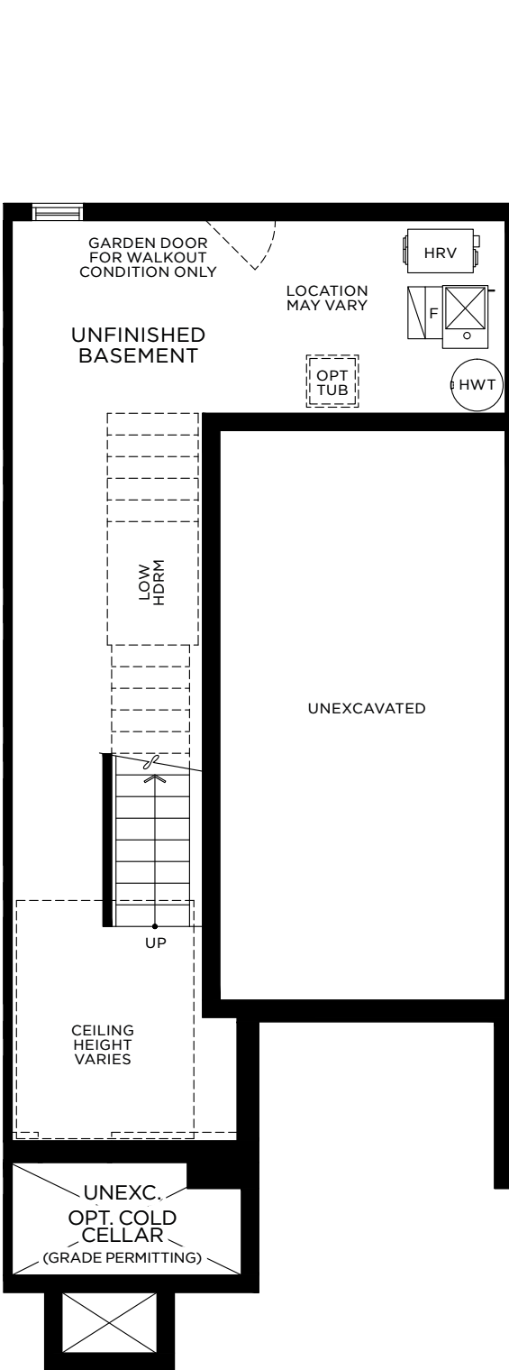
Elevation A2, A, B, B2 Basement
