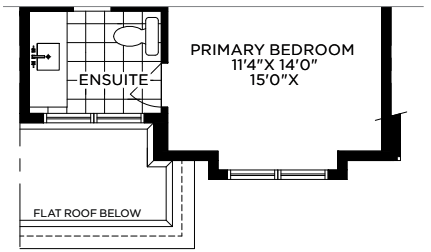
Mod 3 Elev B Upper Floor
