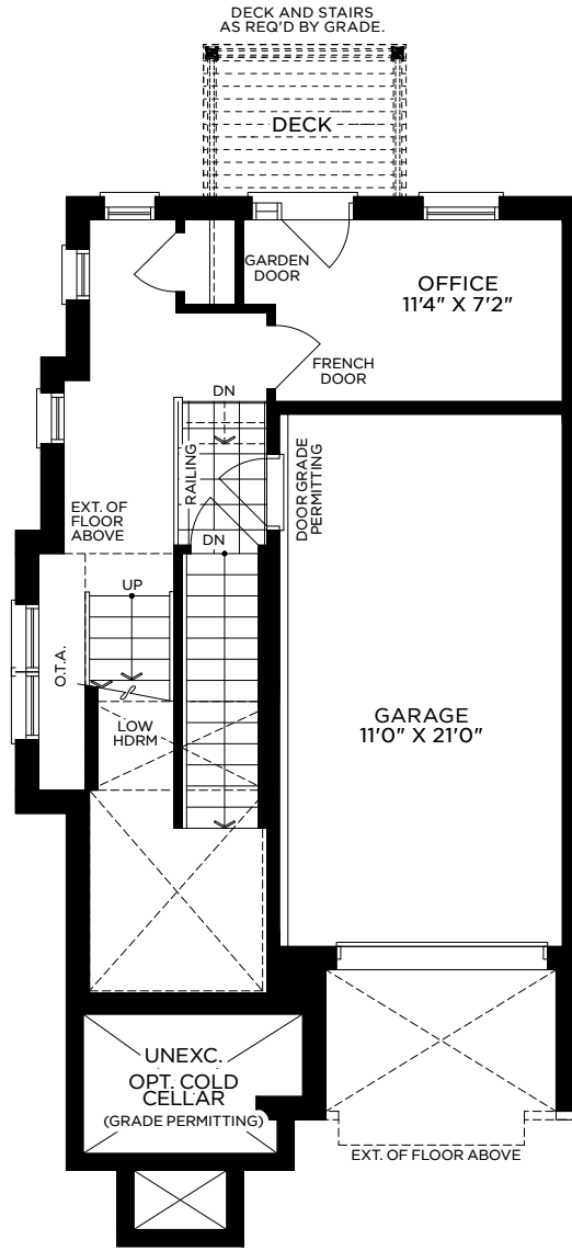
Corner Mod 2 Elev A, B Lower Floor
