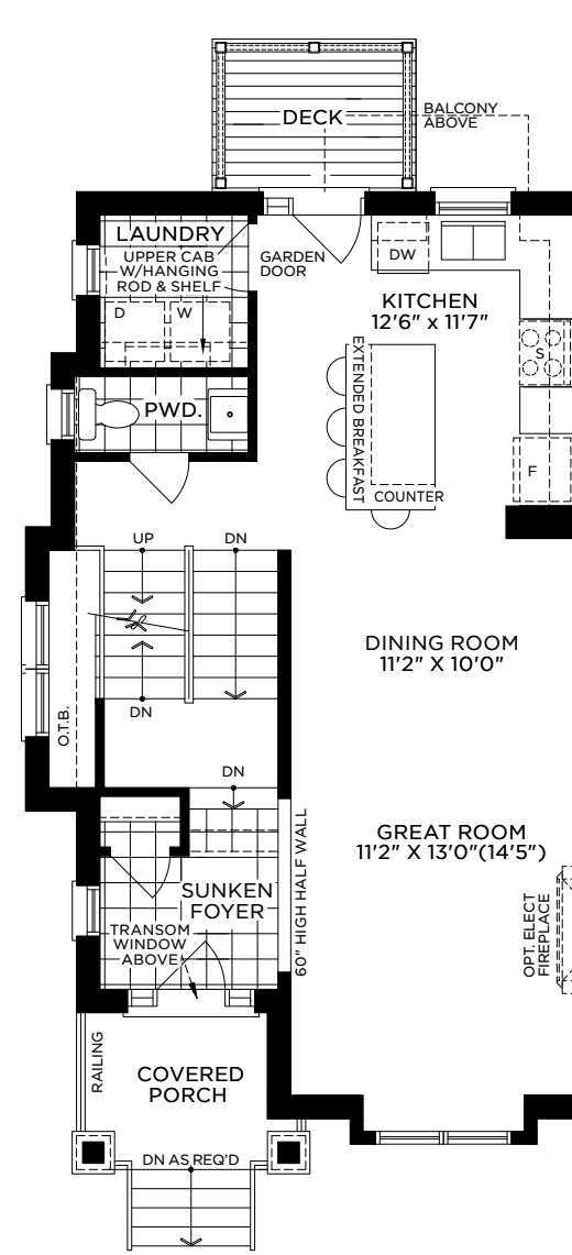
Corner Mod 2 Elev A Main Floor
