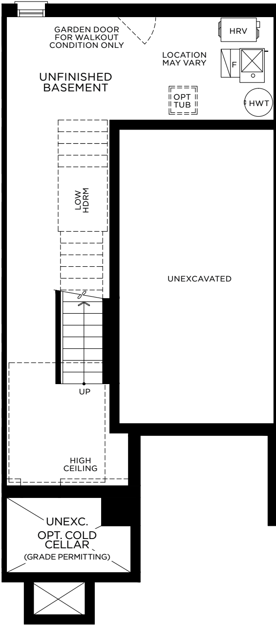
Mod 1 Elev A, B Basement
