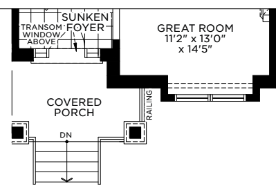
Mod 1 Elev B Main Floor
