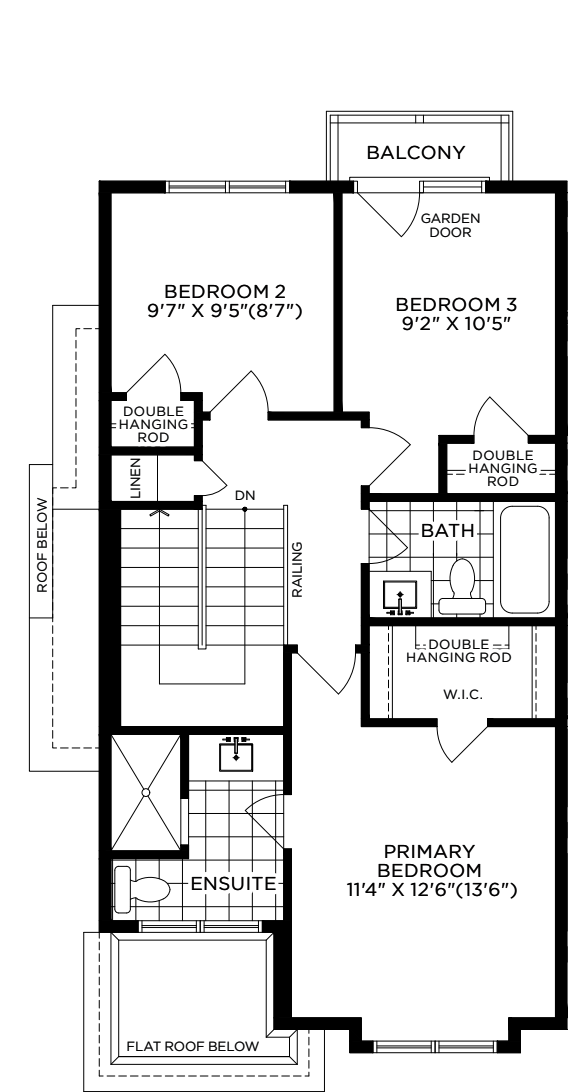
Corner Mod 2 Elev A Upper Floor
