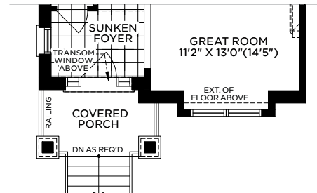
End Mod Elev B Main Floor
