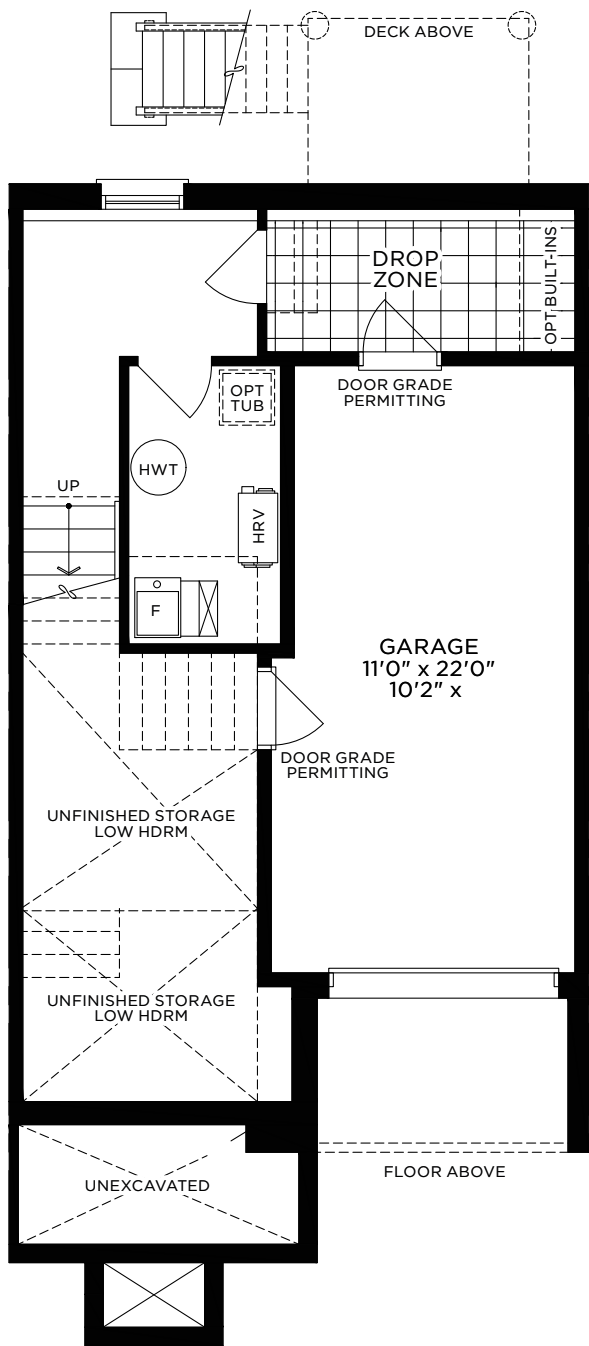
Elevation A2, B2 Lower Floor
