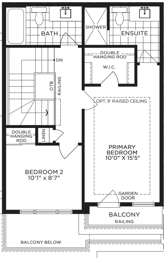
Corner Elev B Optional Upper Floor
