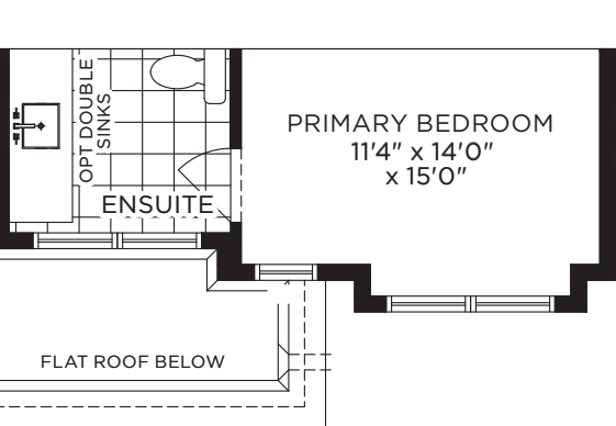
Elevation A, B2 Upper Floor
