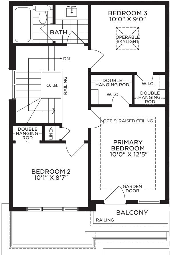
End Elev A Upper Floor
