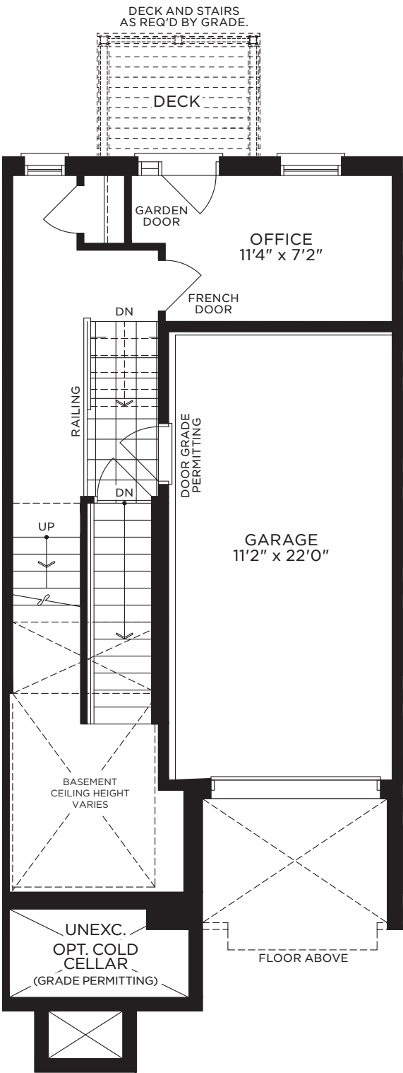
Elevation A2, B Lower Floor
