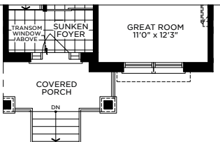
Elevation B3 Main Floor
