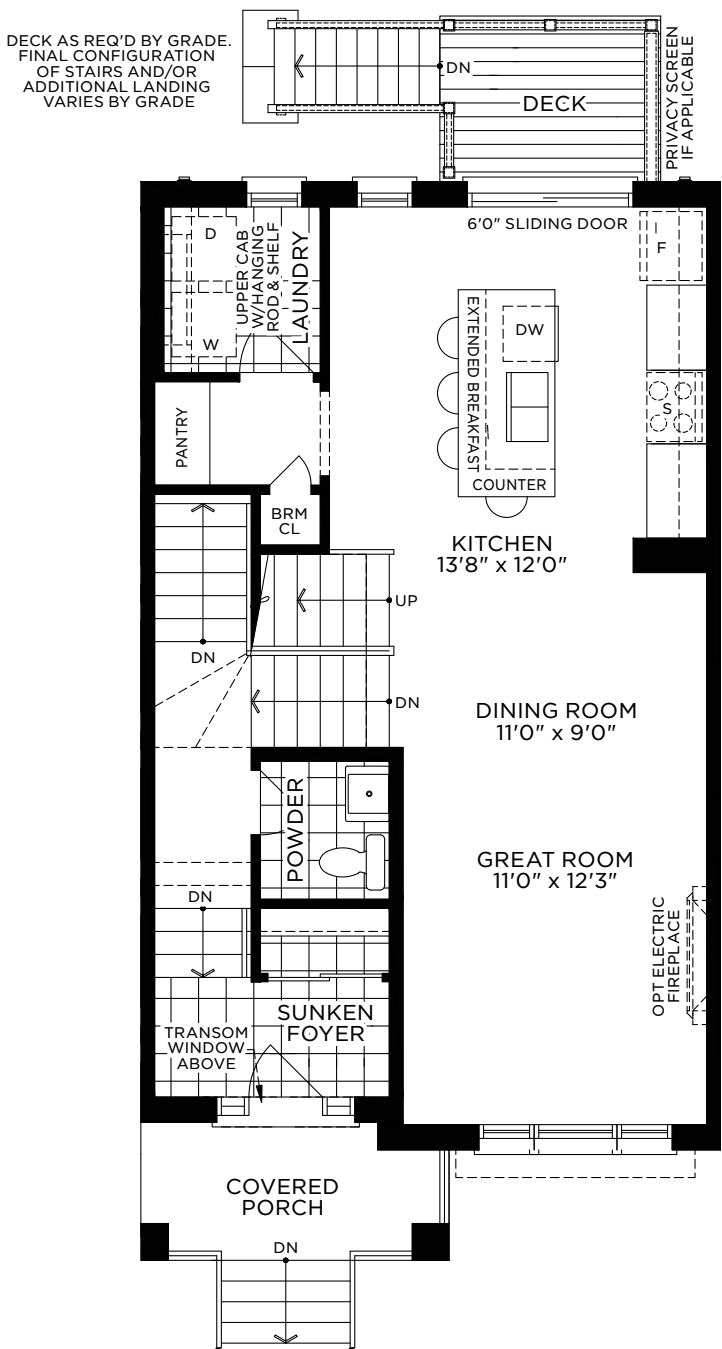
Elevation A Main Floor
