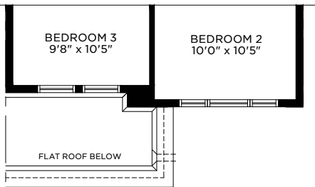
Elevation B Upper Floor
