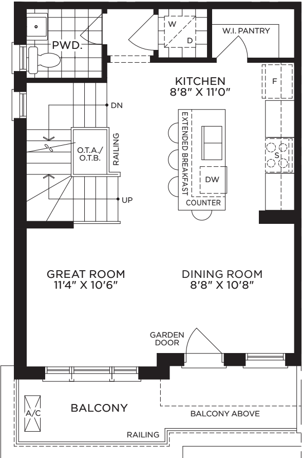
End Elev A Main Floor
